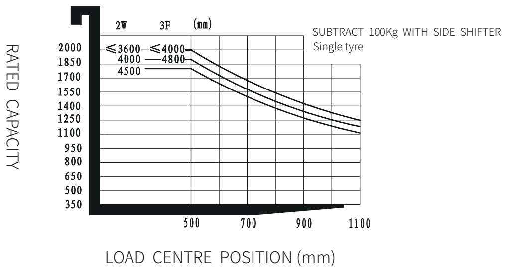
RATED CAPACITIES AND LOAD CENTERES GRAPH
